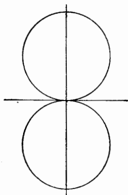
FIG. 2-8. Bidirectional cosine power pattern.
