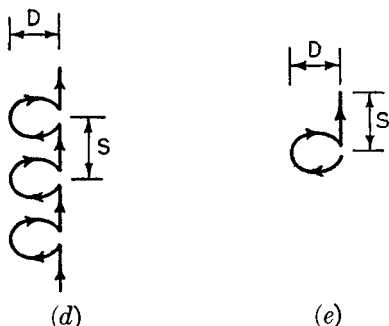
FIG. 7-10(d) and (e). Modified helix for normal mode calculations.
