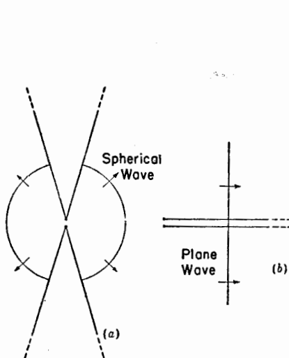
FIG. 8-1. An infinite biconical antenna (a) is analogous to an infinite uniform transmission line (b).
