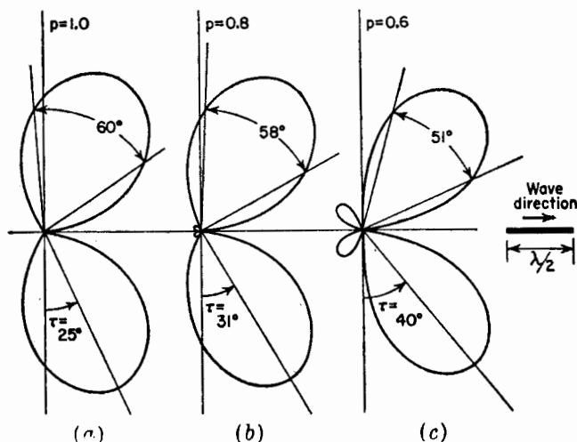
FIG. 5-16. Far-field patterns of linear \frac{1}{2} -wavelength antenna carrying a uniform traveling wave (to right) for three conditions of relative phase velocity ( p = 1.0, 0.8 , and 0.6 ). The tilt angle \tau and the half-power beam widths are indicated for each pattern.
