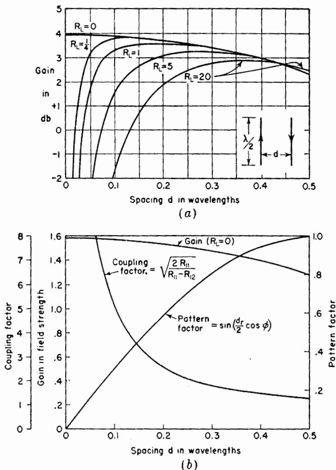
FIG. 11-13. (a) Gain of end-fire array of two out-of-phase \frac{1}{2} -wavelength elements (flat-top beam antenna) with respect to a \frac{1}{2} -wavelength reference antenna as a function of the spacing for five values of the loss resistance R_L . (b) Gain curve for R_L = 0 with variation of its component factors, the coupling factor and the pattern factor, for \phi = 0 .
