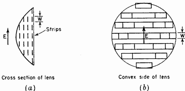
FIG. 14-7. Artificial dielectric lens of flat metal strips.
