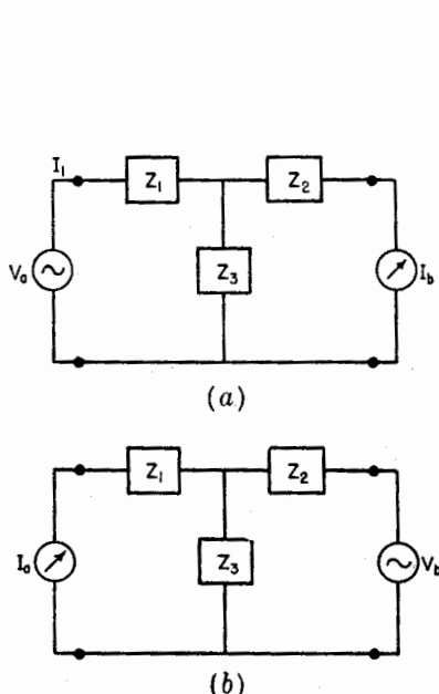
FIG. 10-3. Equivalent circuits used in proof of reciprocity theorem.
