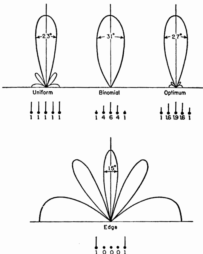
FIG. 4-29. Normalized field patterns of broadside arrays of five isotropic point sources spaced \frac{1}{2} wavelength apart. All sources are in the same phase, but the relative amplitudes have four different distributions: uniform, binomial, optimum, and edge. Only the upper half of the pattern is shown. The relative amplitudes of the five sources are indicated in each case by the array below the pattern, the height of the line at each source being proportional to its amplitude. All patterns are adjusted to the same maximum amplitude.
