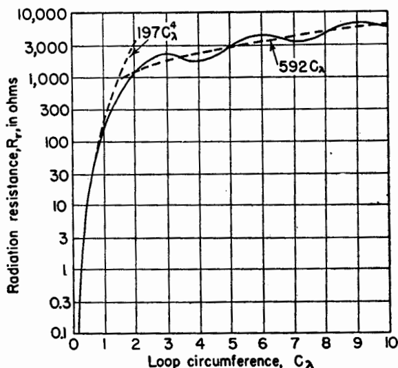
FIG. 6-12. Radiation resistance of single-turn circular loop with uniform, in-phase current as a function of the loop circumference in wavelengths, C_\lambda .
