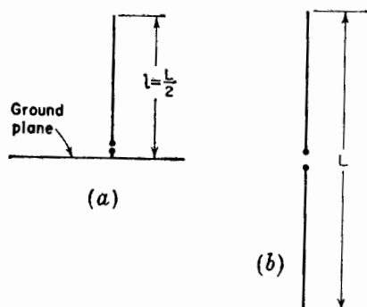
FIG. 10-7. Stub antenna of length l at (a) and center-fed antenna of length L at (b).
