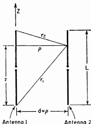
FIG. 10-11. Parallel coupled antennas with dimensions.
