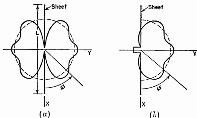
FIG. 13-9. Solid curves show patterns in x - y plane for slot in finite sheet of length L . Slot is open on both sides in (a) and closed on left side in (b). Dashed curves show pattern for infinite sheet. All patterns idealized.
