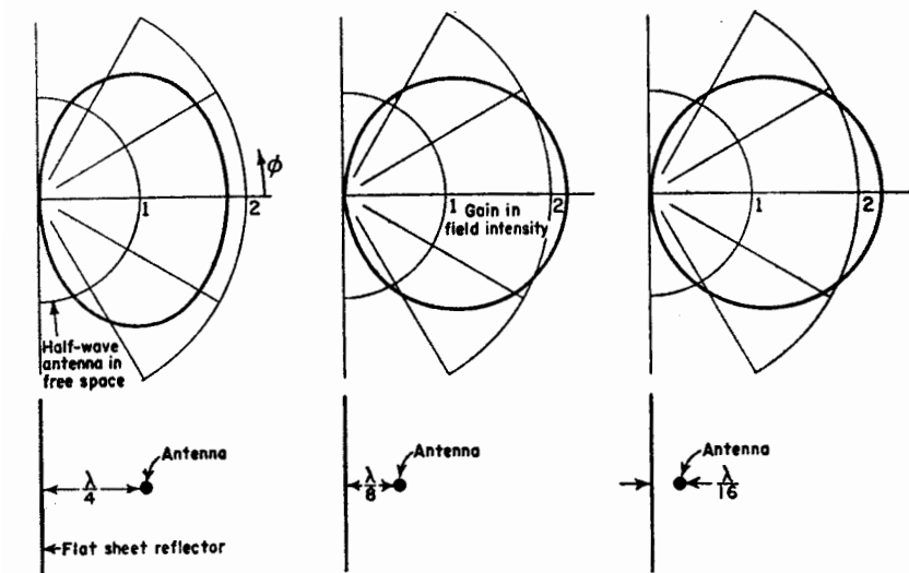
FIG. 12-3. Patterns of \frac{1}{2} -wavelength antenna at spacings of \frac{1}{4} , \frac{1}{8} , and \frac{1}{16} wavelengths from infinite flat sheet reflector. Patterns give gain in field intensity over \frac{1}{2} -wavelength antenna in free space with same power input.
