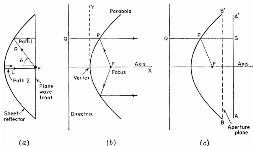
FIG. 12-15. Parabolic reflectors.
