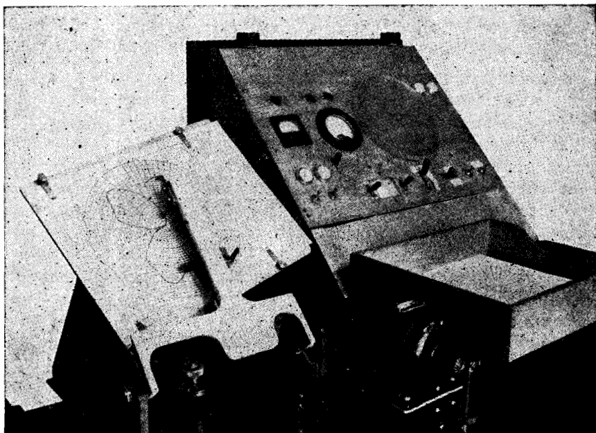
FIG. 15-5. Automatic antenna pattern recorder. The pattern is drawn by a pen on polar coordinate paper. Control equipment is at the right. ( Antenna Laboratory, The Ohio State University. )
