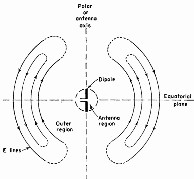
FIG. 1-6. Field configuration near dipole antenna.
