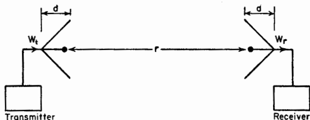
FIG. 15-13. Absolute gain measurements with two identical antennas.
