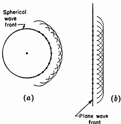
FIG. 4-39. Spherical and plane wave fronts with secondary waves of Huygens.
