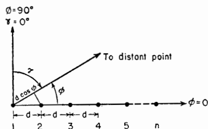
Fig. 4-18. Arrangement of linear array of n isotropic point sources.
