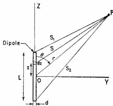
FIG. 5-3. Geometry for short dipole.
