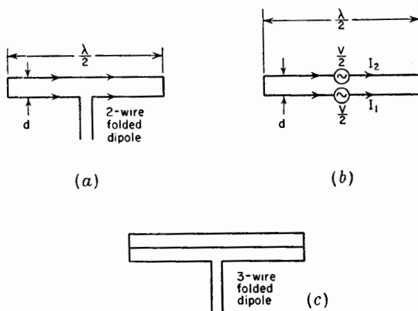
FIG. 14-25. Folded dipoles.
