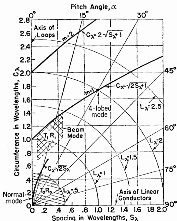
FIG. 7-4. Spacing-circumference chart for helices showing regions for different modes of operation.
