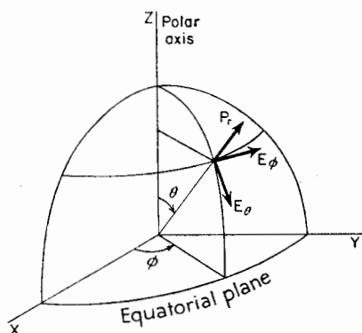
FIG. 2-16. Relation of the Poynting vector and the electric field components of the far field.
