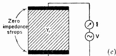
FIG. 13-14. Shunt admittance across transmission line (a) is analogous to infinite screen in path of plane wave (b). Method of measuring surface admittance of screen is suggested in (c).
