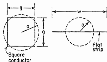
FIG. 9-5. Conductors of square and flat cross section with equivalent circular conductors of radius a .
