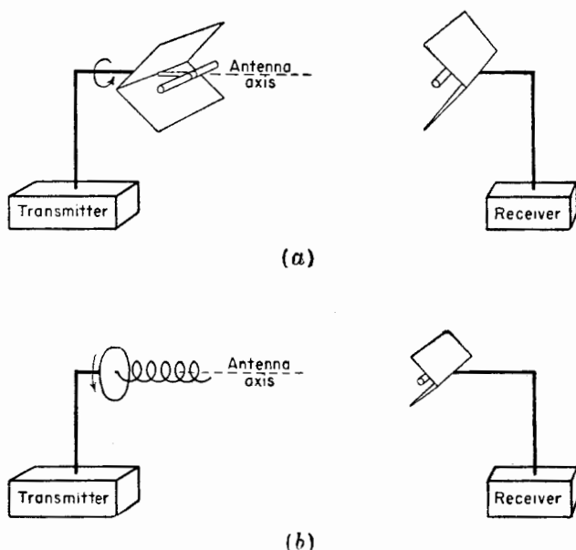
FIG. 15-34. Arrangements for antenna rotation experiments.
