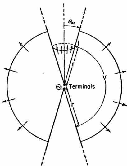
FIG. 8-2. Infinite biconical antenna showing voltage V and current I at a distance r from the terminals.
