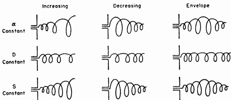
FIG. 7-36. Types of tapered axial mode helical antennas.
