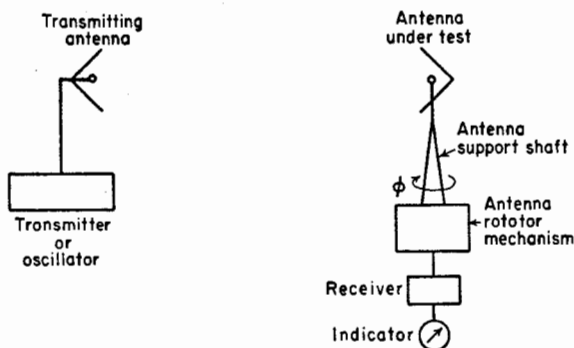
FIG. 15-4. Antenna pattern measuring arrangement.
