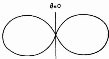
FIG. 2-10. Sine squared power pattern.
