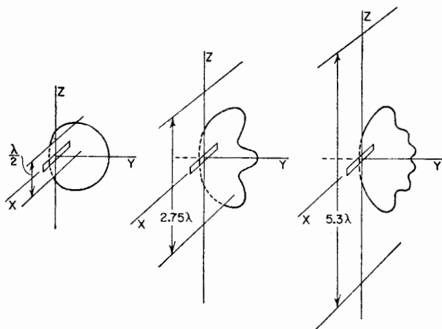
FIG. 13-10. Measured \phi -plane patterns of \frac{1}{2} -wavelength boxed-in slot antennas in finite sheets of three lengths L = 0.5 , 2.75 , and 5.3 wavelengths. The width of the slots is 0.1 wavelength. (After Dorne and Lazarus.)
