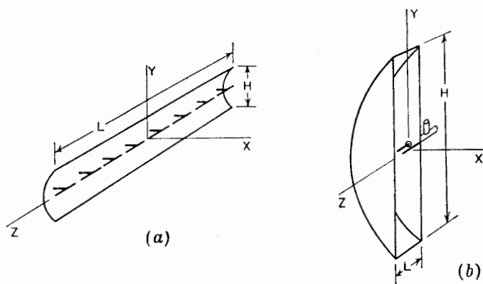
FIG. 12-22. Parabolic reflector with linear array of eight in-phase \frac{1}{2} -wavelength antennas (a) and "pillbox" or "cheese" antenna (b).
