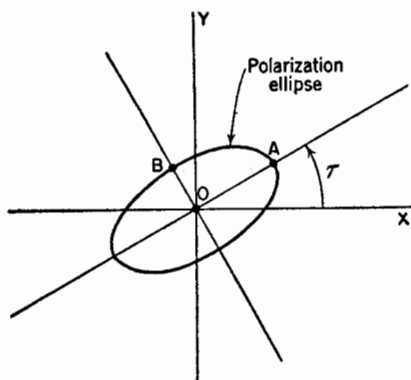
FIG. 15-22. Polarization ellipse.
