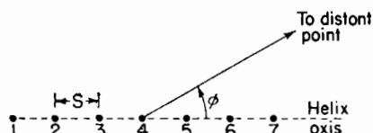
FIG. 7-16. Array of isotropic point sources, each source representing 1 turn of the helix.
