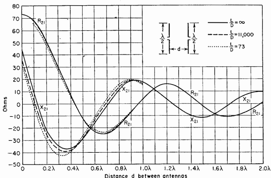
FIG. 10-12. Curves of mutual resistance ( R_{21} ) and reactance ( X_{21} ) of two parallel side-by-side linear \frac{1}{2} -wavelength antennas as a function of distance between them. Solid curves are for infinitesimally thin antennas as calculated from Carter's formulas. Dashed and dotted curves between 0 and 1.0\lambda spacing are from Tai's data for antennas with L/D ratios of 11,000 and 73 respectively.
