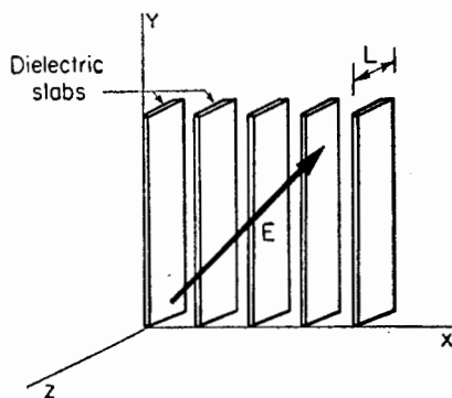
FIG. 14-40. Wave polarizer.
