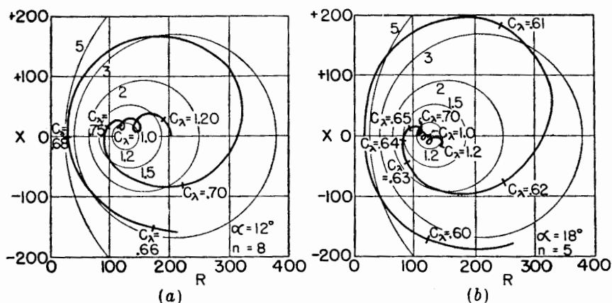
FIG. 7-14. Measured impedance spiral for 12^\circ , 8-turn helix (a) and 18^\circ , 5-turn helix (b). The helices are of fixed physical size. The impedance (resistance R and reactance X , in ohms) is shown as a function of frequency, the circumference in wavelengths at a given frequency being indicated at intervals along the spirals.
