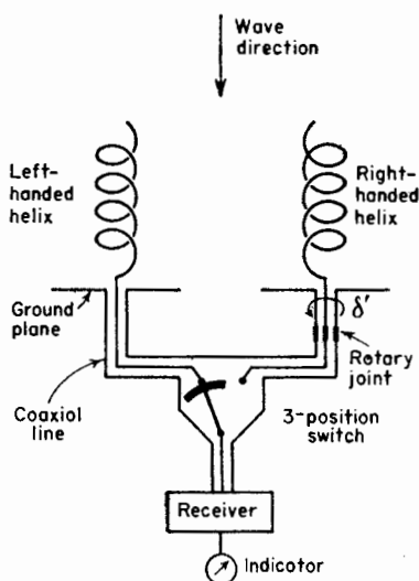
FIG. 15-32. Arrangement for measuring left and right circular components of wave and phase angle \delta' between them in circular component method.
