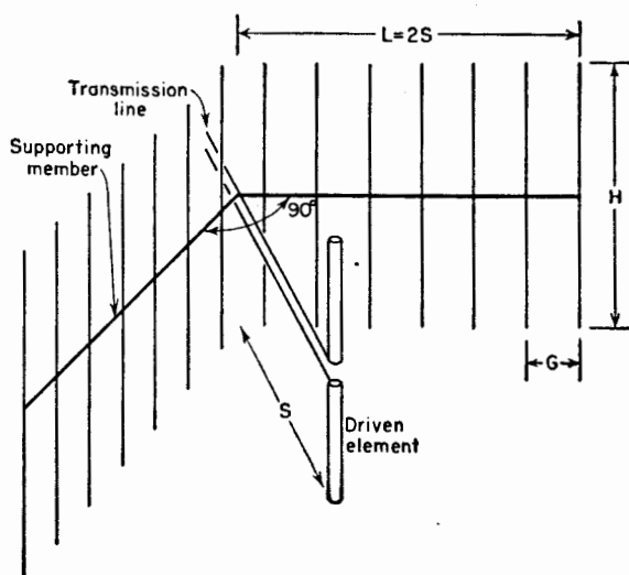
FIG. 12-13. Grid-type reflector.
