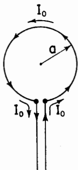
FIG. 6-11. Loop and transmission line.
