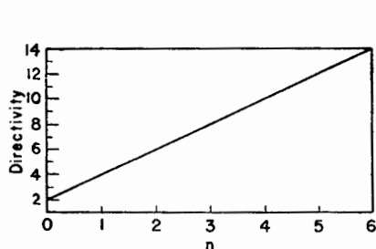
FIG. 2-13. Directivity vs. n for unidirectional sources with \cos^n \theta power patterns.
