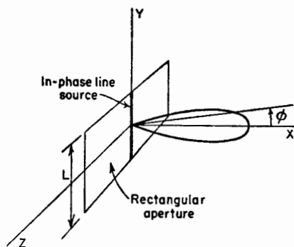
FIG. 12-24. Line source of height L and rectangular aperture of height L .
