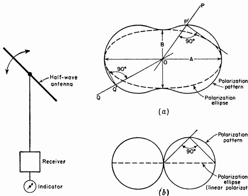
FIG. 15-29. Schematic arrangement of rotatable linearly polarized antenna for measuring polarization pattern.
