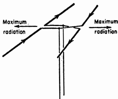
FIG. 11-14. Flat-top beam antenna with closely spaced elements carrying equal out-of-phase currents.
