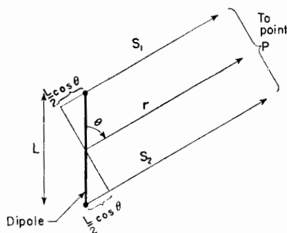
FIG. 5-4. Relations for short dipole when r \gg L .
