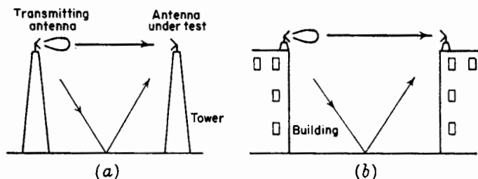
FIG. 15-8. Antenna test setups.
